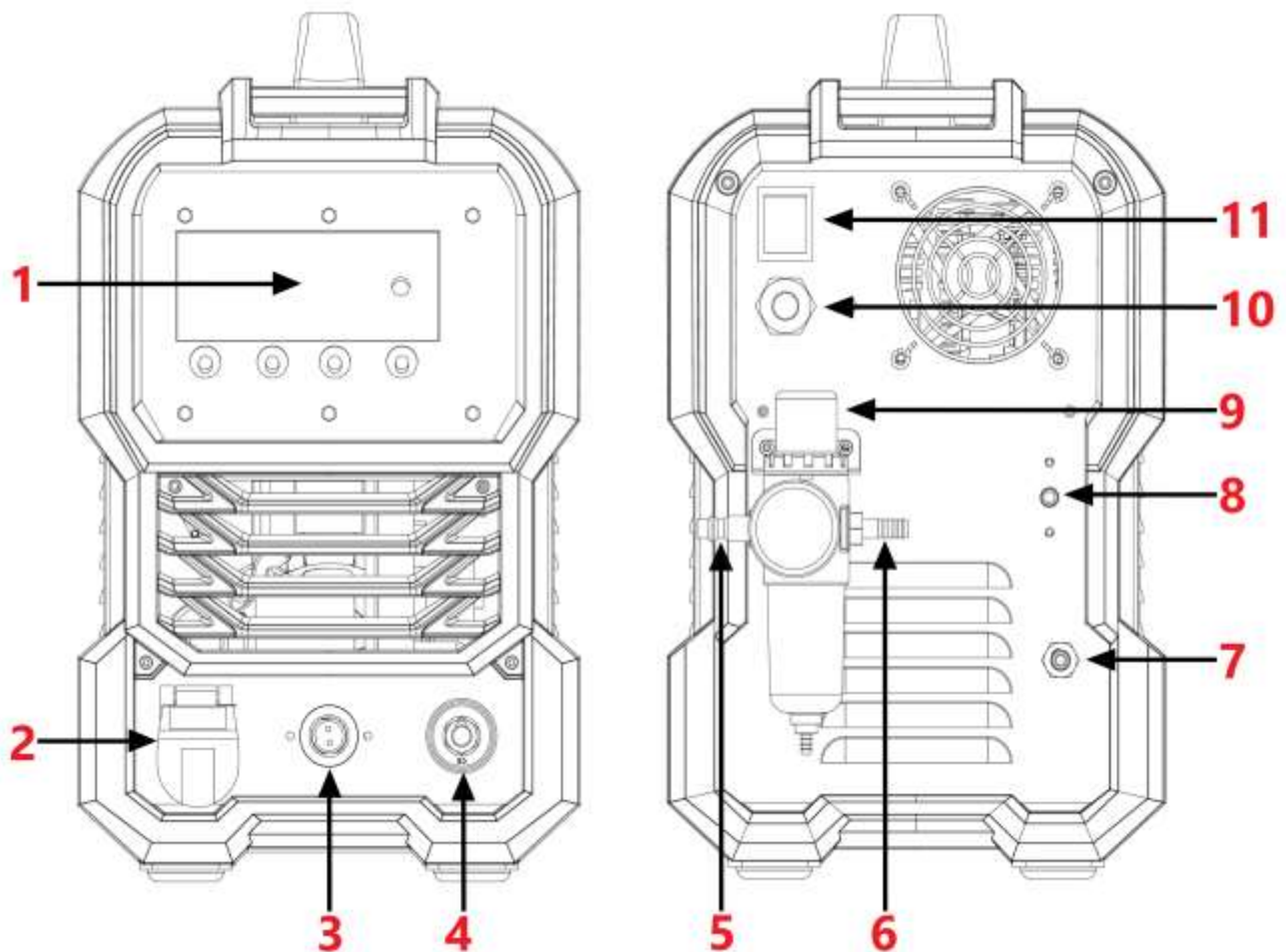
Figura 2 – Vista frontal e traseira Joy CUT 45 AIR.
