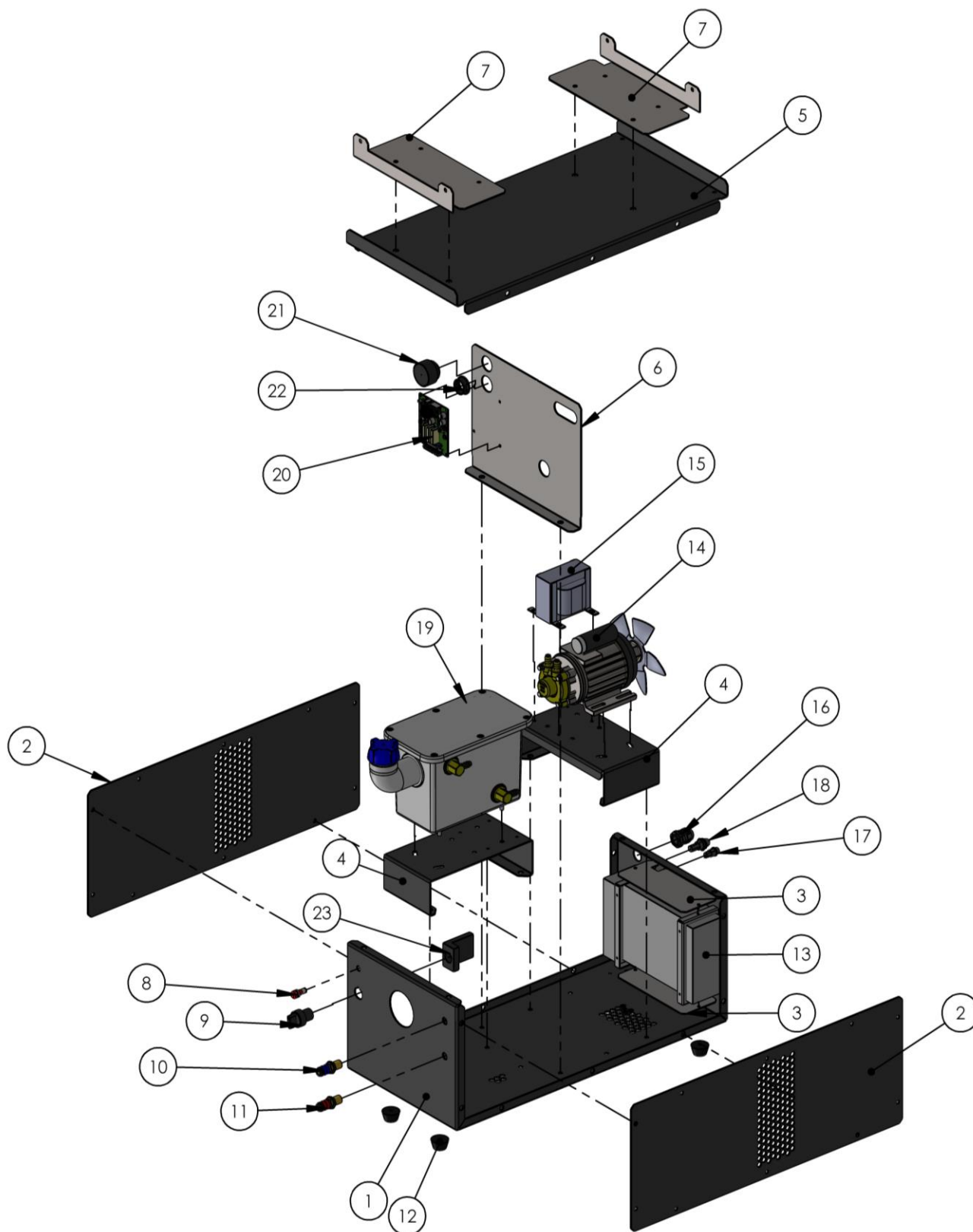
Figura 9 – Vista explodida SRB 315 smart.
