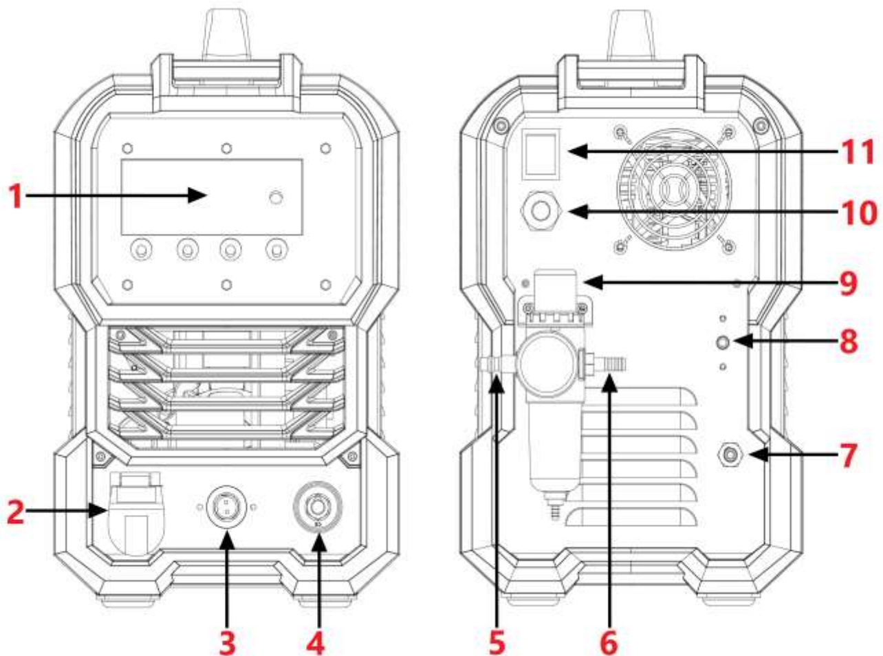
Figura 2 – Vista frontal e traseira Joy CUT 45 AIR.
